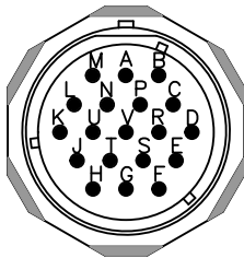
FRONT VIEW 19 PIN CONTACT (MALE)
