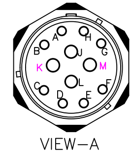
FRONT VIEW 12PIN SOCKET (FEMALE)
